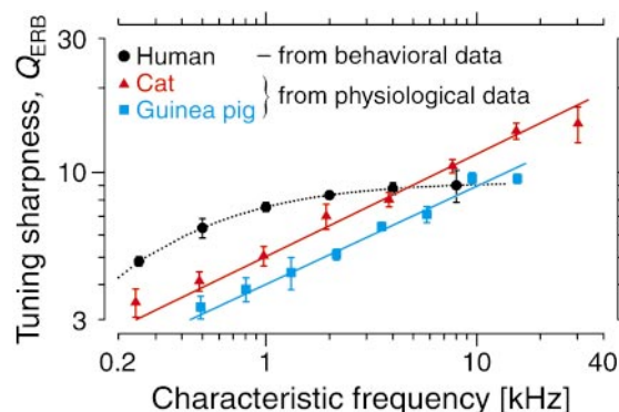
Fig. 1. Sharpness of cochlear tuning in three species derived from previous measurements. Q_{\text{ERB}} is the ratio \text{CF}/\text{ERB}(\text{CF}) , where CF is the characteristic (or center) frequency of the filter, and ERB is the equivalent rectangular bandwidth. The cat and guinea-pig Q_{\text{ERB}} values were computed from threshold frequency tuning curves of single auditory-nerve fibers (12, 13) by using standard algorithms (14). The human Q_{\text{ERB}} curve was computed from Glasberg and Moore's polynomial fit to a variety of standard psychophysical masking data (15, 16). Their formula gives Q_{\text{ERB}}(\text{CF}) = (Q_{\infty} \cdot \text{CF} / (\text{CF} + \text{CF}_{1/2})) , where the parameters Q_{\infty} = 1,000[\text{Hz}] / (4.37 \cdot 24.7[\text{Hz}]) = 9.26 and \text{CF}_{1/2} = 1,000[\text{Hz}] / 4.37 = 230 \text{ Hz} . The symbols with error bars represent the means and standard errors computed from the original data in logarithmically spaced frequency bins. The straight lines show power-law fits to the animal data (see Table 1). The flattening of the Q_{\text{ERB}} at the highest CFs—visible in the guinea pig above 15 kHz and perhaps in the cat above 20 kHz—may well be a measurement artifact. Mechanical responses in the high-frequency region of the cochlea are extremely labile, and cochlear tuning at high CFs can easily be damaged (e.g., as a result of trauma caused by surgically opening the auditory bulla).
